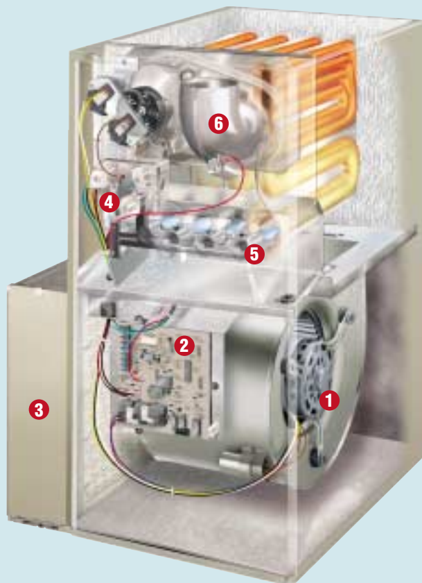
Model 312 shown with Bryant High Efficiency Media Filter - Sold Separately
